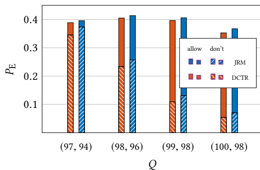
Figure 6: Detection error P_E of SI-UNIWARD at 0.4 bpnzac in DC images when modes with q_{kl}^{(1)} = q_{kl}^{(2)} are/are not allowed for embedding. BOSSbase+BOWS2 dataset.
